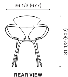
REAR VIEW
